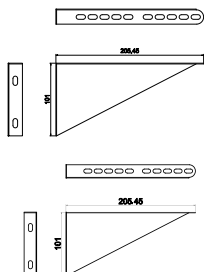
Mounting bracket for square chute
