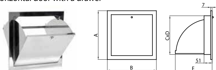
Horizontal door with a drawer
